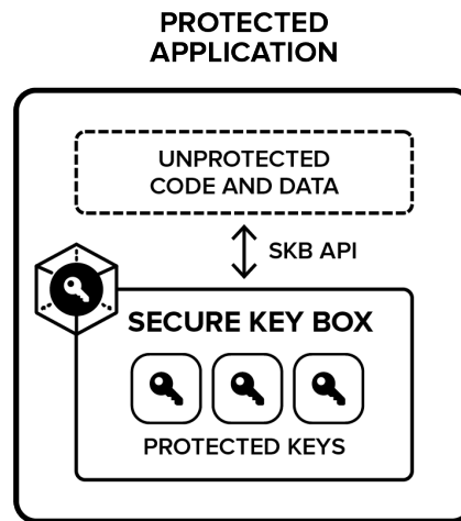
Figure 4: Applying SKB protection to the target application
