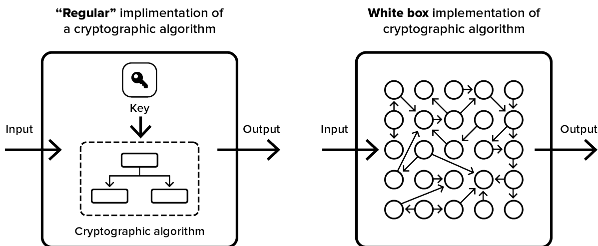
Figure 3: Unobfuscated implementation versus white box implementation
